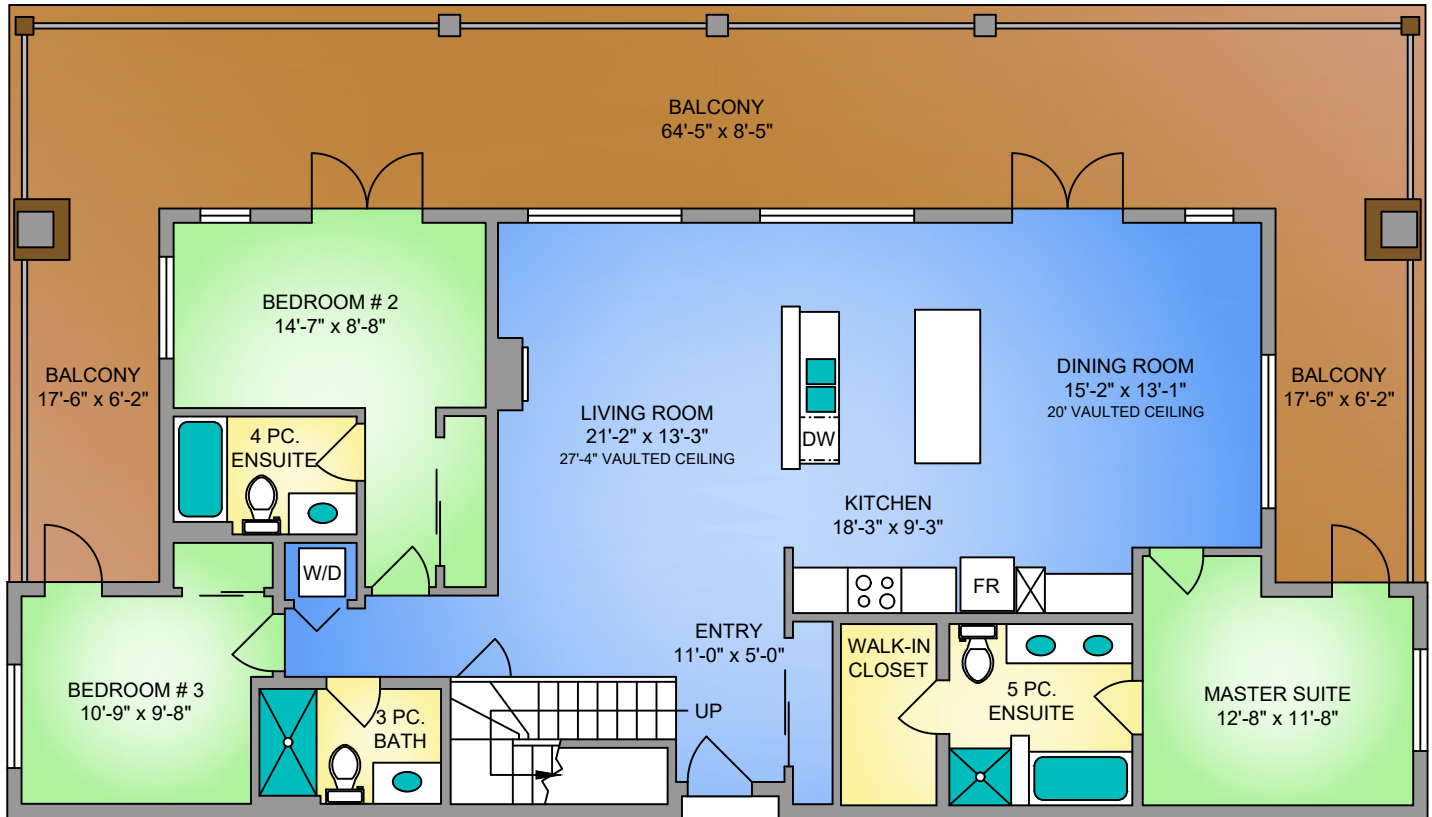
MAIN FLOOR 1587 SQ. FT. 10' CEILING
